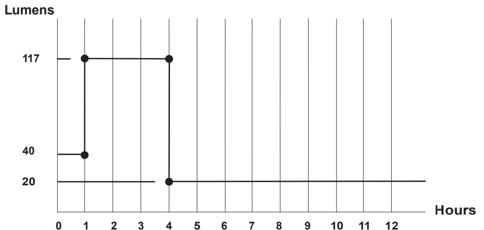
LUMENS/WORKING TIME
